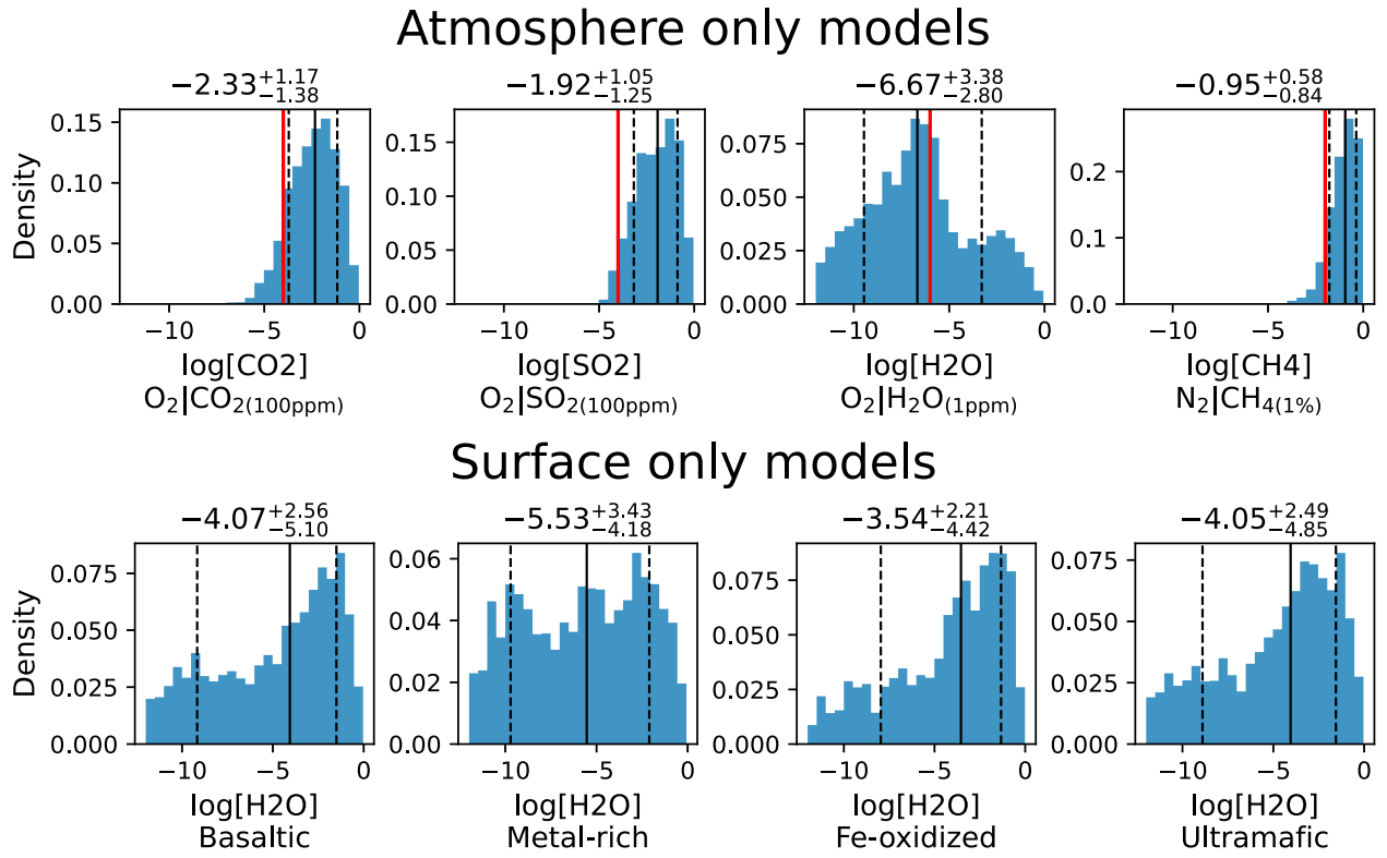
Figure 11. Top: Posterior distributions of the retrieved volume mixing ratios of \text{CO}_2 , \text{SO}_2 , \text{H}_2\text{O} , and \text{CH}_4 using atmospheric forward models without a nongray surface. The retrieved mean and 1\sigma width is given on top of each panel and shown with black solid and dashed vertical lines. The input mixing ratio (the “true” value) is shown as a red vertical line. The atmospheric composition used in the forward model is listed below the horizontal axis label. All atmospheric species are recovered in the retrieval, although the retrieved mixing ratio tends to be somewhat overpredicted for \text{CO}_2 , \text{SO}_2 , and \text{CH}_4 . Bottom: Posterior distributions of the retrieved \text{H}_2\text{O} volume mixing ratios from the surface-only (no atmosphere) forward models. The surface crust used in the forward model is listed below the horizontal axis label. The basaltic, iron-oxidized, and ultramafic surfaces lead to a relatively pronounced posterior distribution that may erroneously be interpreted as a weak detection of atmospheric \text{H}_2\text{O} .
