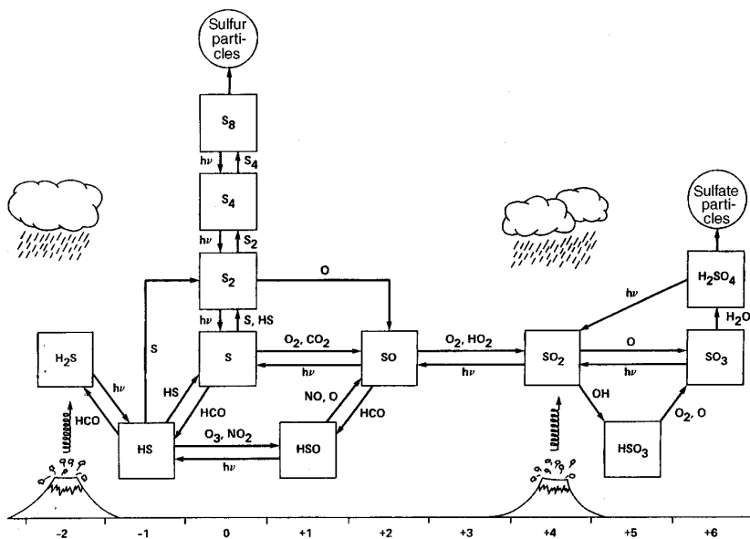
Figure 9 Diagram illustrating sulfur photochemistry in a low- \text{O}_2 atmosphere. The horizontal scale is the sulfur-oxidation state. Sulfur is outgassed as either \text{SO}_2 or \text{H}_2\text{S} . It leaves as one of a variety of soluble sulfur gases or as solid \text{S}_8 particles. Mass-independent fractionation patterns created by photochemical reactions (e.g., \text{SO}_2 photolysis) can be preserved under such circumstances but not in an \text{O}_2 -rich atmosphere. (From Kasting et al. 1989).
