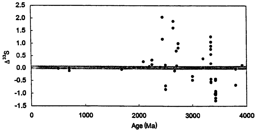
Figure 8 Sulfur-isotope ratios measured in rocks of different ages. Shown on the vertical scale is \Delta^{33}\text{S} , which represents the deviation of the ^{33}\text{S} abundance from its usual relationship to ^{32}\text{S} and ^{34}\text{S} . Not shown are 73 rock samples of Phanerozoic age ( < 0.54 Ga), all of which have \Delta^{33}\text{S} values equal to 0 \pm 0.1\% . Photochemical reactions in a low- \text{O}_2 atmosphere are required to produce nonzero \Delta^{33}\text{S} values. [From Farquhar, Bao & Thiemans (2000). Reprinted with permission of Science magazine.]
