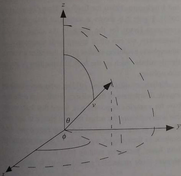
Figure 5.5 The geometry for Jeans' escape of a molecule with velocity v , in spherical polar coordinates, where \theta is zenith angle and \phi is azimuthal angle.
