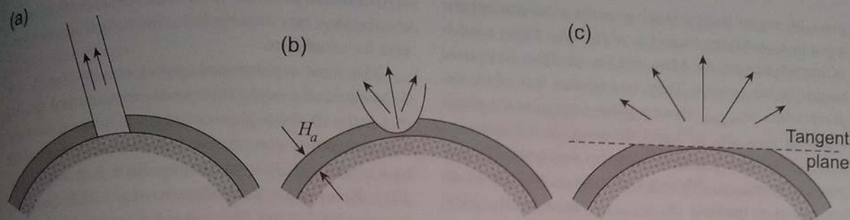
Figure 5.19 Various semi-analytical approximations to atmospheric impact erosion. (a) In the cookie-cutter approximation, the mass of gas that escapes is similar to that intercepted by the impactor multiplied by a factor close to unity (Walker, 1986). (b) In the massless point explosion approximation, an accelerating shock wave drives off the atmosphere of scale height (Ahrens, 1993). (c) In the tangent plane model of atmospheric impact erosion, a sufficiently massive impactor removes the entire atmosphere above a plane tangent to the planet. The impactor is required to have an impact velocity above a threshold of twice the escape velocity of the target (Melosh and Vickery, 1989).
