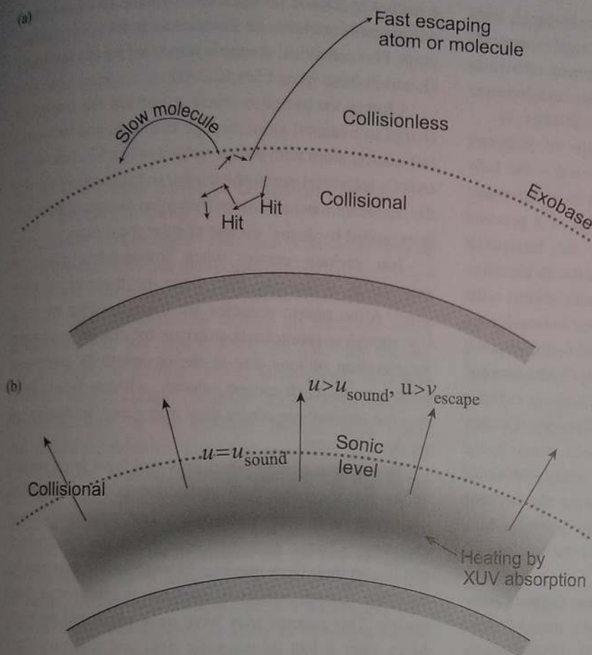
Figure 5.2 Schematic diagram of thermal escape end-members. (a) Jeans' escape is escape of molecules or atoms with an upward-directed component of velocity bigger than the escape velocity from the collisional part of the atmosphere into a virtually collisionless exosphere. (b) Transonic hydrodynamic escape is where the upper atmosphere has sufficient heating to produce a radial outward velocity u , at the speed of sound ( u_{\text{sound}} ) in the collisional part of the atmosphere at the radius labeled sonic level . Heating is typically by soft x-rays and extreme ultraviolet radiation (EUV). The atmosphere flows out to the vacuum of space driven by a pressure gradient (with the boundary condition set at the sonic level) and the supersonic flow reaches escape velocity, v_{\text{escape}} . At very high levels, the atmosphere will have very few collisions and the fluid assumption of hydrodynamic escape breaks down. However, under the transonic circumstances depicted, the fluid equations extrapolated to infinity provide a reasonable approximation to the density, temperature, and flow profiles.
