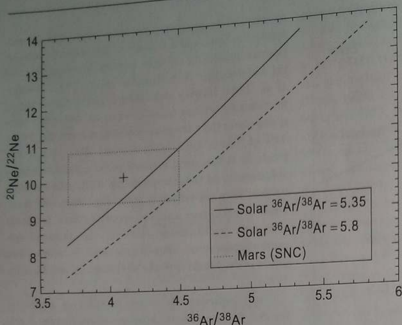
Figure 5.18 The ^{20}\text{Ne}/^{22}\text{Ne} ratio produced in fractionating argon by hydrodynamic escape from Mars, assuming an initial ^{20}\text{Ne}/^{22}\text{Ne} of 13.7. (From Fig. 7 of Zahnle (1993).)
