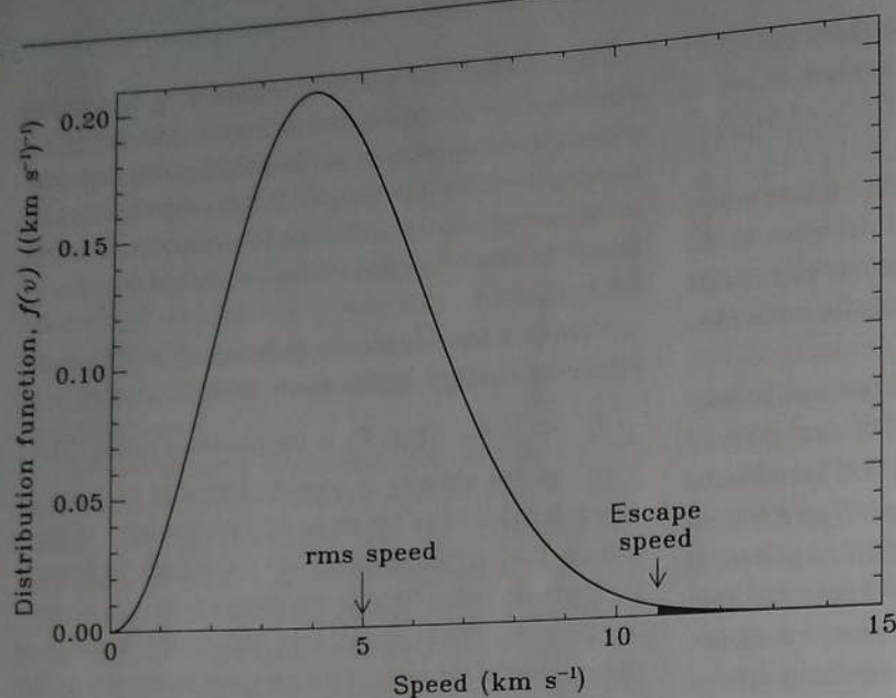
Figure 5.3 The Maxwell-Boltzmann speed distribution function f(v) , for hydrogen atoms at 1000 K. The escape speed at Earth's exobase and the root mean square (rms) speed of the atoms are indicated. Only those atoms in the energetic tail of the speed distribution with speeds exceeding the escape speed (shaded) are able to undergo Jeans' thermal escape . In contrast, atoms with the most probable speed at the peak of the distribution, or with the slightly higher rms speed, are unable to escape.
