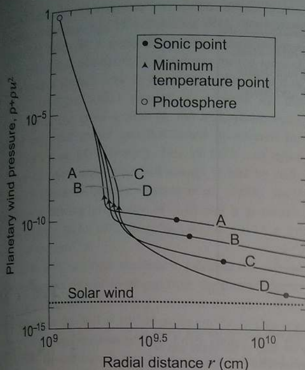
Figure 5.12 Transonic hydrodynamic escape model results from Sekiya, M. et al. (1980a, b) for a primordial \text{H}_2 -rich atmosphere showing the pressure ( p + \rho u^2 ) of the planetary wind as a function of distance. The four cases A–D have a net absorbed solar EUV flux of 1, 0.1, 0.01, and 0.001 \text{W m}^{-2} , respectively. This flux is absorbed in the outer atmosphere through ionization of \text{H}_2 where it heats the gas and drives hydrodynamic escape. The photosphere is a much lower altitude level where solar visible light is assumed to be absorbed and mostly reemitted in thermal infrared, so that it is not available to drive escape. Expansion of the atmosphere with increasing flow velocity typically causes a minimum temperature point, marked by triangle ( \blacktriangle ). The sonic level ( \bullet ) typically has a higher pressure than today's solar wind pressure, which is marked with a dashed horizontal line. (From Sekiya, M. et al. (1980). Reproduced with permission. Copyright 1980, The Physical Society of Japan.)
