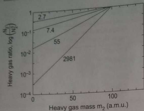
Figure 5.16 The evolution of the inventory of heavy gas 2 relative to its initial inventory as a function of molecular mass, m_2 . For this graph, a constant crossover mass of 100 is assumed and a constant hydrogen escape flux. The numbers on the diagonal lines indicate values of N_0^1/N_1 , which shows the depletion of the lighter gas inventory. Thus the lines at the bottom of the plot correspond to later times in an evolutionary history. (Adapted from Hunten et al. (1987).)
