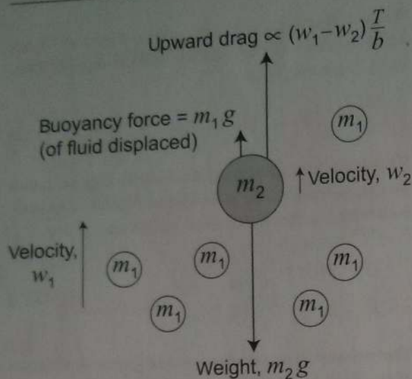
Figure 5.15 The forces acting on a heavy gas molecule of mass m_2 moving at an upward velocity w_2 immersed in a light gas flowing upwards in the diffusively separated upper atmosphere. The light gas has molecules of mass m_1 that move at an upward velocity of w_1 . Absolute temperature is T and b = Dn where D is the diffusion coefficient and n is total number density. If the initial total upward force on molecule 2 is greater than the downward force of its weight minus buoyancy, molecule 2 will be accelerated until the upward and downward forces come into balance.
