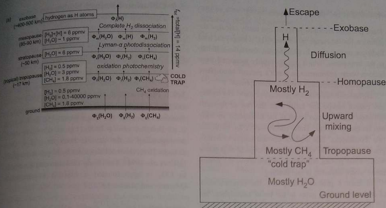
Figure 5.9 (a) A schematic diagram of hydrogen-bearing species in Earth's atmosphere showing processes responsible for the profiles shown in Fig. 5.8(b). Hydrogen is input from the ground in fluxes ( \Phi ) of water, hydrogen and methane. At the tropical tropopause, a cold trap limits the flux of hydrogen from water vapor into the stratosphere. The total H mixing ratio f_T , just below the homopause sets the diffusion-limited escape flux of hydrogen to space ( \Phi_e ), which is reflected by f_T in the lower stratosphere above the tropical tropopause cold trap. (b) A schematic diagram showing the two principal "bottle-necks" for hydrogen escape: the tropical tropopause cold trap and diffusion above the homopause.
