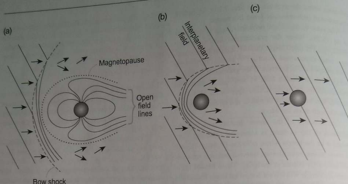
Figure 5.7 (a) Interaction of the solar wind with a planet that has a significant magnetic field, e.g. Earth (and similar also for Jupiter, Mercury, Saturn, and Uranus). Inside the magnetopause, the magnetic field is dominated by that of the planet and solar wind particles that are thermalized at the bow shock (where the wind is brought to rest) flow around the magnetopause and have little influence on the atmospheric evolution. Open field lines, however, allow ions to escape from the poles if they exceed the escape velocity. (b) Interaction of the solar wind with a planet without a significant magnetic field, e.g. present-day Mars or Venus. A bow shock is formed much closer to the planet due to an induced field in the ionosphere. Thermalized solar wind particles can interact directly with the atmosphere. (c) The solar wind collides directly with a body that has low electrical conductivity, no ionosphere/atmosphere, and no magnetic field, e.g. the Moon. (Adapted from Fig. 3.8 in Lewis and Prinn (1984).)
