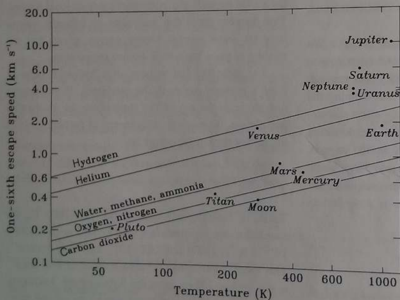
Figure 5.4 A schematic graph showing gas species that are prone to undergo thermal escape from planets in the Solar System on the basis of the "rule of thumb" approach discussed in the text. For bodies with substantial atmospheres, the temperature corresponds to the average exobase temperature. For the Moon and Mercury, the temperature is the mean surface temperature. The sloping lines correspond to the root mean square speed of the various gas molecules at the given temperature.
