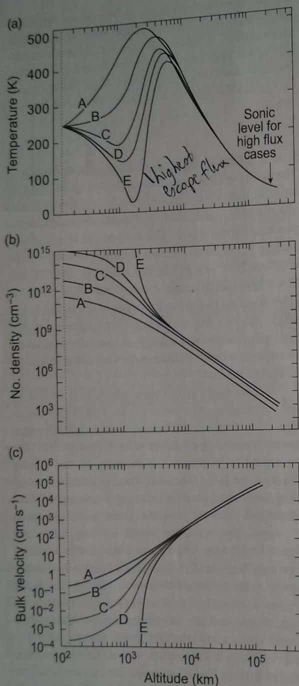
Figure 5.14 Temperature (a), number density (b), and upward velocity (c) versus altitude for a transonically escaping pure atomic H terrestrial atmosphere. (After Watson et al. (1981).). The sonic level is shown by the arrow in panel (a) at 2 \times 10^5 km or \sim 30 planet radii. An EUV heating efficiency of 0.15 was assumed in the calculations. The escape fluxes (H atoms \text{cm}^{-2} \text{s}^{-1} ) for the five cases, normalized to the Earth's surface, are: (A) 5.7 \times 10^{10} , (B) 2.2 \times 10^{11} , (C) 2.9 \times 10^{11} , (D) 3.1 \times 10^{11} , and (E) 3.5 \times 10^{11} . The escape flux for case E is close to the energy-limited escape flux.
