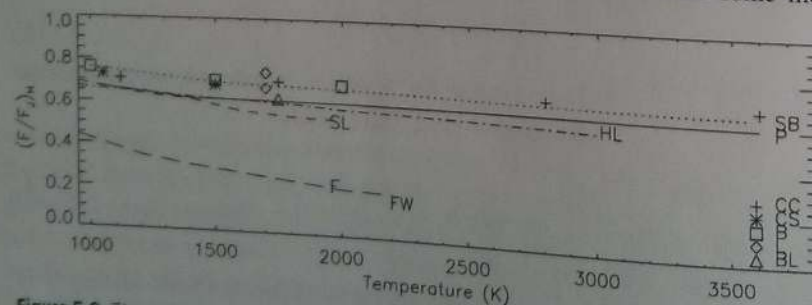
Figure 5.6 The ratio of the non-Maxwellian escape flux of hydrogen, F , to the Maxwellian Jeans' escape flux, F_J , versus the temperature at the Earth's exobase (from Pierrard, 2003). The solid line (P) shows the results of Pierrard (2003). Results are compared with those obtained with Monte Carlo simulations represented by different symbols: CC (Chamberlain and Campbell, 1967); L (Lew, 1967); B (Brinkmann, 1970); CS (Chamberlain and Smith, 1971); BL (Barakat and Lemaire, 1990). The other lines correspond to analytic solutions: HL (Hays and Liu, 1965); F (Fahr, 1976); FW (Fahr and Weidner, 1977); SL (Shizgal and Lindenfeld, 1980); SB (Shizgal and Blackmore, 1986).
