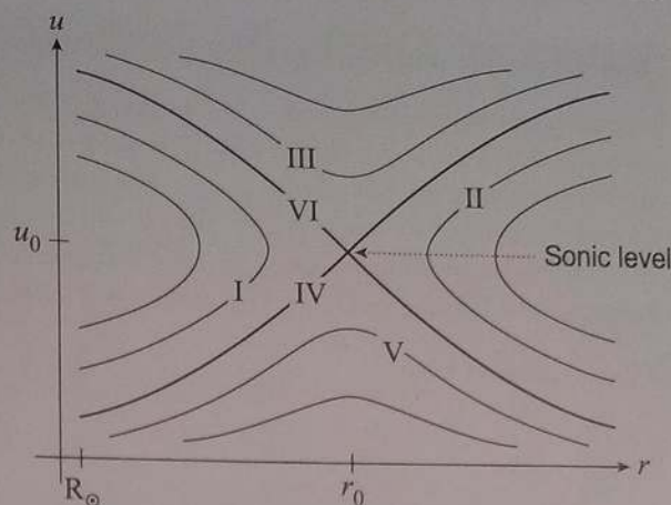
Figure 5.11 Solutions to the isothermal, time-independent, hydrodynamic escape equations (Box 5.2, eqs. (B5.11) or (B5.12)), but for an ionized gas. Six different classes of solution are shown (I to VI). Solution IV, which increases in speed and passes through the sonic level (also called the critical point) and becomes supersonic, is the solar wind solution. (Following Parker (1963).)
