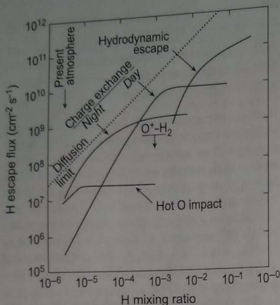
Figure 5.10 Calculated hydrogen escape fluxes from Venus. From left to right: increasing H concentrations to ~1% eventually permit hydrodynamic escape. At lower concentrations of H, charge exchange processes are the dominant source of hot H atoms. However, in all cases, the rate of escape is limited by diffusion through the atmosphere from lower layers (dashed line). (From Kumar et al. (1983).)
