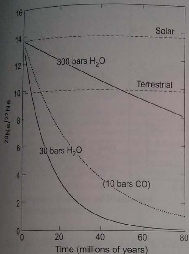
Figure 5.17 Neon isotope fractionation produced by hydrodynamic escape of hydrogen in various steam atmospheres during accretion of the Earth. Three cases are shown. The calculated timescale for neon fractionation is consistent with the expected lifetime of impact-induced steam atmospheres on early Earth. (From Fig. 15 of Zahnle et al. (1990).)
