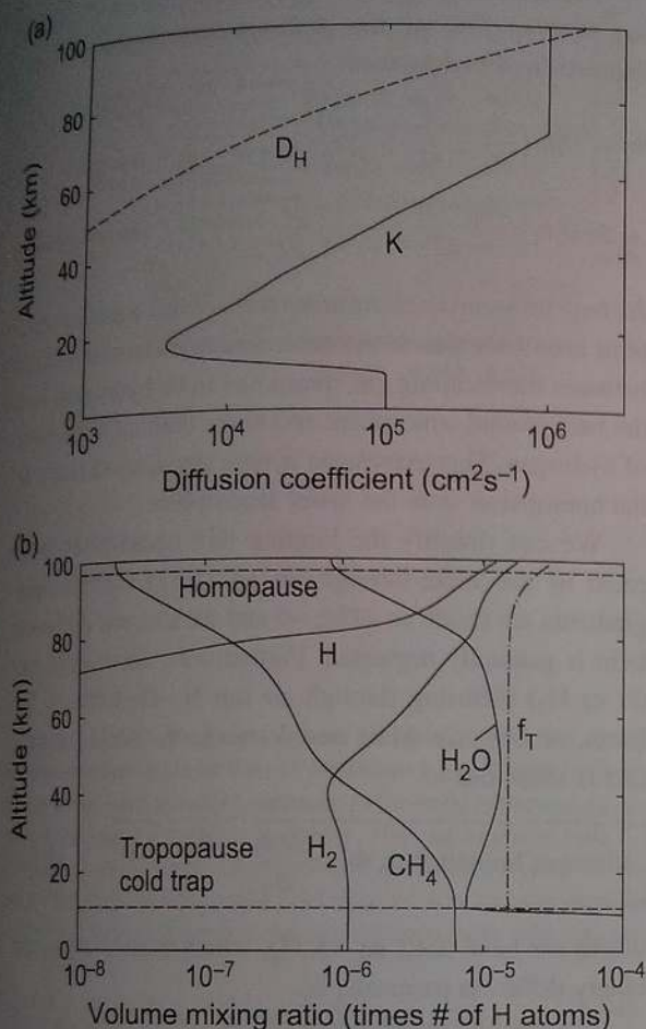
Figure 5.8 (a) Vertical profiles of the eddy diffusion coefficient, K , and the molecular diffusion coefficient for atomic hydrogen, D_H . (b) Vertical mixing ratio profiles of major hydrogen-bearing species, weighted by the number of H atoms in each species, e.g., methane at ground level is 1.8 \text{ ppmv} \times 4 = 7.2 \text{ ppmv H} . The curve labeled f_T represents the total hydrogen mixing ratio defined in the text. The value of f_T begins to increase near the homopause because of diffusive separation of species that favors H and \text{H}_2 .
