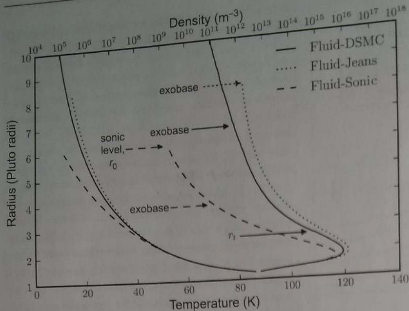
Figure 5.13 Comparison of simulations of atmospheric escape from Pluto with models using a single component, N_2 , for solar-medium conditions at 32 AU. Curves on the left map to the upper axis of number density. Curves on the right map to the left vertical axis, which shows radial distance in number of Pluto radii. The radius of Pluto is 1153 km. Solid lines show a fluid-“direct simulation Monte Carlo” model, where fluid and DSMC methods are coupled at radius r_0 at a Knudsen number of 0.1. This model has an escape rate of 2.6 \times 10^{27} N_2 molecules s^{-1} . Dashed lines show a hydrodynamic escape model, where fluid equations have been applied despite a sonic level above the exobase (Strobel, 2008a). This model has an escape rate of 2.5 \times 10^{27} N_2 molecules s^{-1} but produces inaccurate number density and temperature profiles. Dotted lines show a model with an upper boundary of classical Jeans escape, which has an escape rate of 2.6 \times 10^{27} N_2 molecules s^{-1} . (Modified with permission from Johnson et al. (2013d).)
