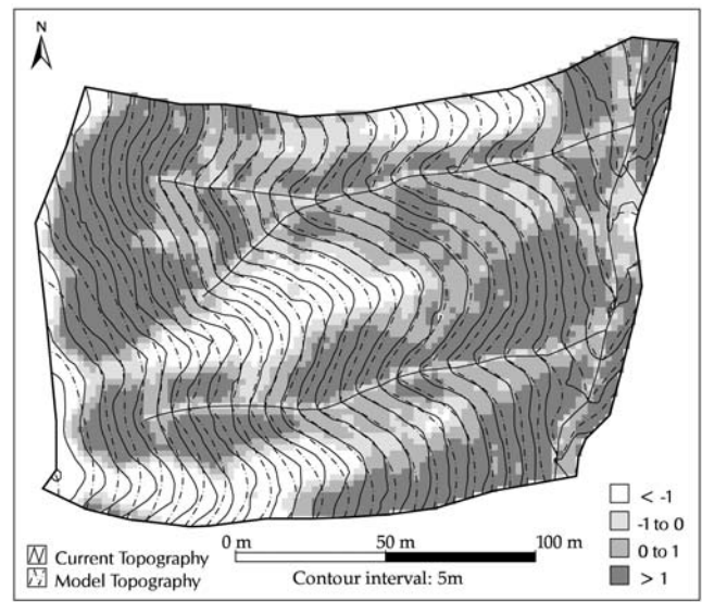
Figure 13. Topographic change for a portion of the study area, showing the initial and final (after one million years) contours and a map of the net difference in elevation (after adding back the total channel lowering to the one million year contour lines). Generally the sharp irregular ridges are lowered and broadened and the broad concavities bordering the channel are narrowed and the elevation increased.
