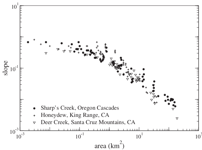
Figure 4. Plot of valley drainage area vs. slope for Sharp's Creek, Oregon, Deer Creek, Santa Cruz Mountains, and Honeydew River, King Range, California. These data, collected by hand from 1:24,000 contour maps, require more than a single power law (e.g., stream power law) because they curve at slopes above \sim 3 -10%. Despite large differences in erosion rate between the sandstone-floored rivers, Deer Creek at \sim 0.2 mm/a [Perg et al., 2000] and Honeydew at \sim 4 mm/a [Merritts and Vincent, 1989], the data define very similar relationships.
