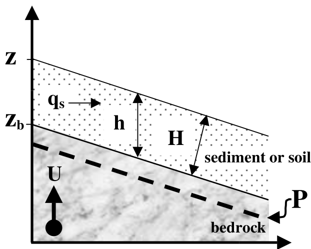
Figure 5. Cartoon illustrating terms in conservation of mass expression (equation 1) for a soil-mantled hillslope or sediment-mantled channel with a ground surface elevation of z . The soil or sediment thickness is h , and uplift, U , is shown as positive upward. Dashed line below soil-bedrock interface illustrates the depth of bedrock converted to soil over a given time period (e.g. soil production rate, P ). The sediment transport per unit hillslope width is q_s . The normal depth, H , and the elevation of the soil-bedrock boundary, z_b , used in equation (11) are also shown.
