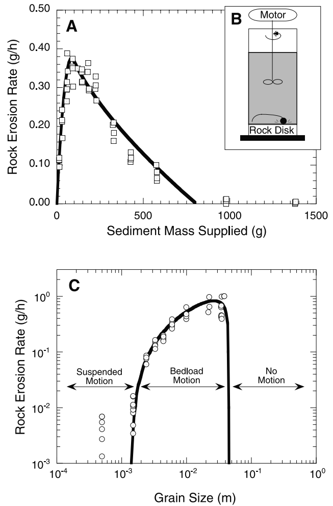
Figure 10. Experimental results demonstrating sediment supply and grain size effects on rates of bedrock wear, shown in grams per hour (g/h). A. Variation in wear rate with sediment supply using the apparatus shown in B. Erosion rate increases with sediment additions until bed armoring by immobile sediment reduces the area of exposed bedrock. Erosion rate declines with further sediment additions until bed is fully buried. C. Wear rate variation with grain size. Wear rate declines with decreasing grain size because of a tendency for small grains to go into suspension and reaches a peak at a grain size that is just above the threshold of motion.
