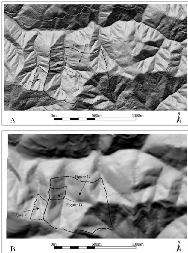
Figure 11. Shaded relief maps of a portion of the Oregon Coast Range near Coos Bay. A. Map based on 2.5-m data density derived from airborne laser swath mapping. B. Map of identical area as A., derived from 10-m grids created from digitized 40-foot contour lines provided by the U.S. Geological Survey. Also shown are the boundaries of the landscape used in the numerical model (and reported in Figure 12), location of a detailed area shown in Figure 13, and the area used to document curvature-slope relationships (Figure 7).
