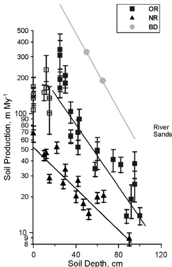
Figure 9. The soil production functions for three sites. These data bracket the entire data set of 7 sites reported in Heimsath [1999]. The Nunnock River area (NR), southeastern Australia [Heimsath et al., 2000], had the lowest production rate for a given soil thickness, with \epsilon_0 = 53 m/my, \alpha = -0.02 (1/m). Sites at Point Reyes, California [Heimsath 1999], \epsilon_0 = 81 m/my, \alpha = -0.016 (1/m) and Frogs Hollow, southeastern Australia [Heimsath et al., 2001b], \epsilon_0 = 141 , \alpha = -0.042 , lie between the Nunnock River and Oregon Coast Range [Heimsath et al. 2001a], \epsilon = 268 , \alpha = -0.03 . Data from the San Gabriel Mountains were similar to the Oregon Coast Range, i.e. \epsilon = 318 , \alpha = -0.038 . Oregon (OR) production rates for shallow samples and exposed bedrock samples (open squares) were not used in the regression. See text for further discussion. The soil production rates at all sites except Black Diamond Mine (BD) were determined by using concentrations of in situ produced cosmogenic nuclides as described in Heimsath et al. [1999]. The two values at BD were derived from garden variety ^{10}\text{Be} in soils [McKean et al., 1993] and suggest \epsilon = 2078 , \alpha = -0.037 .
