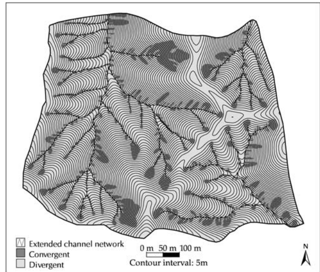
Figure 12. Maps of total topographic convergence or divergence after one million years of constant channel incision. Channel network used is an extension of the current channels to account for effects of debris flow scour. Time step was 1 year. Field calibrated parameters used in equation (10) are K_{nl} = 0.0032 \text{ m}^2/\text{yr} and S_c = 1.25 [Roering et al. , 1999]. To convert to a mass flux we multiplied the right hand side of (10) by the soil bulk density ( \rho_s = 800 \text{ kg/cm}^3 ). Field calibrated parameters used in equation (11) are \epsilon_0 = 0.000268 \text{ m/yr} , \alpha = -0.03 \text{ (1/m)} [Heimsath et al. , 2001]. In this case, to convert to mass flux, we multiplied the left hand side of equation (11) by the rock bulk density ( \rho_r = 2270 \text{ kg/m}^3 ) and the right hand side by the soil bulk density. Note the convergent areas above the channel head and upslope of irregularities in channel paths.
