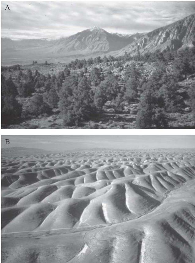
Figure 1. A. View of the eastern side of the Sierra Nevada Mountains, California (Mt. Tom near Bishop). B. Soil-mantled, ridge and valley topography near Salinas, California
