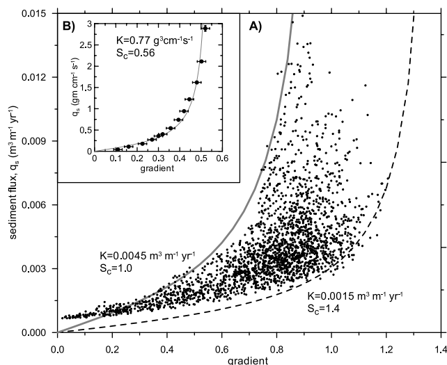
Figure 8. A. Plot of sediment flux versus local hillslope gradient derived from high resolution topographic data in the Oregon Coast Range [from Roering et al. , 1999]. Parameters reported are best-fit estimates of equation 10 in the text. B. Measured sediment flux versus gradient derived from acoustically-disturbed sandbox experiments [ Roering et al. , 2001]. Line passing through data is for the best fit values of equation 10.
