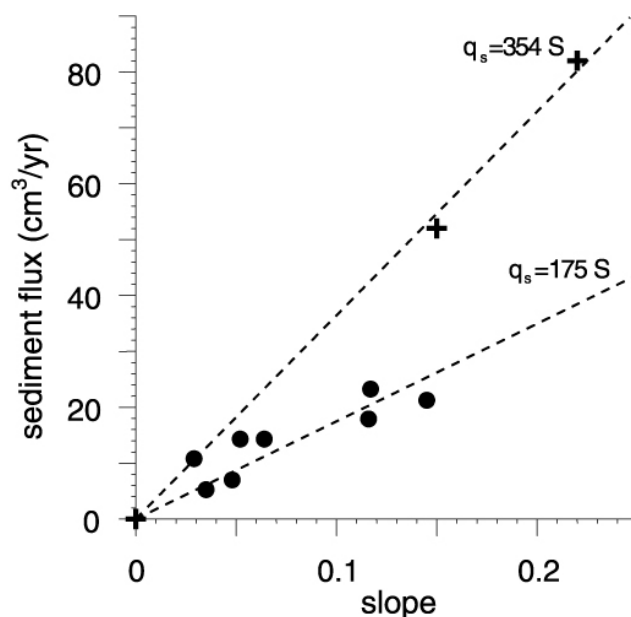
Figure 6. Plot of slope versus soil flux rate for sites in a clay-rich soil in coastal California (crosses; from McKean et al., 1993 ) and an alpine hillslope in the Wind River Range, Wyoming (infilled circles; from Small et al., 1999 ). Data from both sites (acquired using cosmogenic radionuclides)
