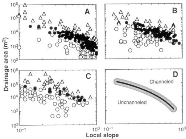
Figure 2. Drainage area and local slope for channel heads (solid dots), unchanneled valleys upslope from the channel heads (circles), and low-order channels (triangles) from: A. coastal Oregon (adjacent to the area represented in Figures 4 and 5), B. northern California, and C. southern California. D. summarizes general finding that there is a area-slope topographic threshold distinguishing channeled and unchanneled areas. This threshold also corresponds to the boundary between hillslopes and channeled valleys (from Montgomery and Dietrich, 1992).
